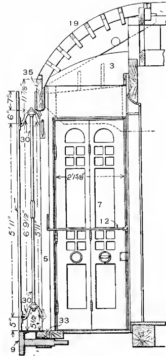
Fig. 2429. Sectional Side View.
